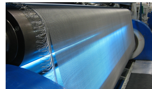
Stainless steel mesh is cut, pre-treated, and powder coated
